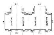
EXTERIOR BUILDING DIMENSIONS SCALE: 1" = 20'
