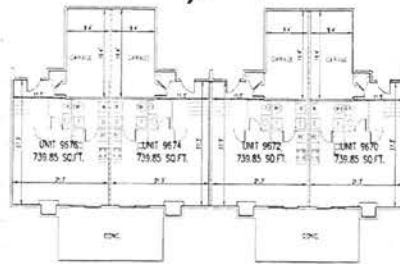
LOWER LEVEL FLOOR ELEVATION=96.71 CEILING ELEVATION=95.78 GARAGE ELEVATION=95.84
