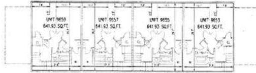
SECOND FLOOR FLOOR ELEVATION=9724 CEILING ELEVATION=9834
