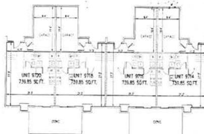
LOWER LEVEL FLOOR ELEVATION=950.30 CEILING ELEVATION=958.20 GARAGE ELEVATION=951.90
