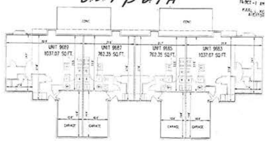
FIRST FLOOR FLOOR ELEVATION=96.11 CEILING ELEVATION=95.13 GARAGE ELEVATION=90.25
