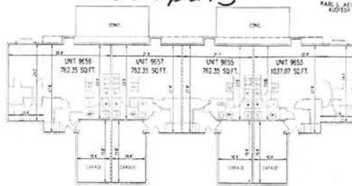
FIRST FLOOR FLOOR ELEVATION=9658 CEILING ELEVATION=9718 GARAGE ELEVATION=9674
