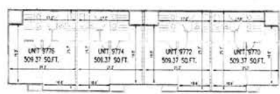
UPPER LEVEL FLOOR ELEVATION=90.00 CEILING ELEVATION=90.00
