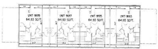
SECOND FLOOR FLOOR ELEVATION=97.36 CEILING ELEVATION=97.36
