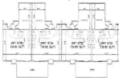
LOWER LEVEL FLOOR ELEVATION=90.00 CEILING ELEVATION=90.00 GARAGE ELEVATION=90.00
