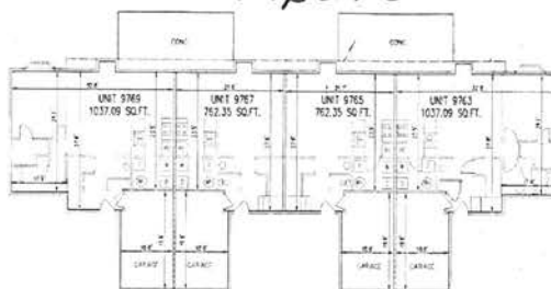
FIRST FLOOR FLOOR ELEVATION=95.726 CEILING ELEVATION=95.12 GARAGE ELEVATION=95.37
